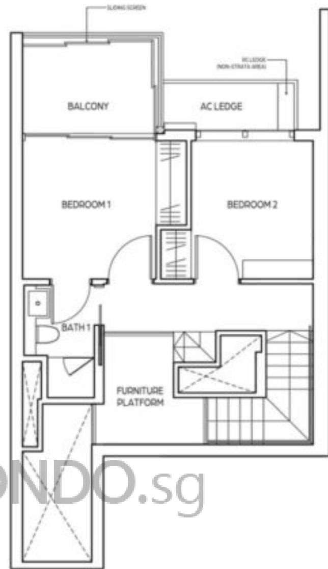
UPPER FLOOR
