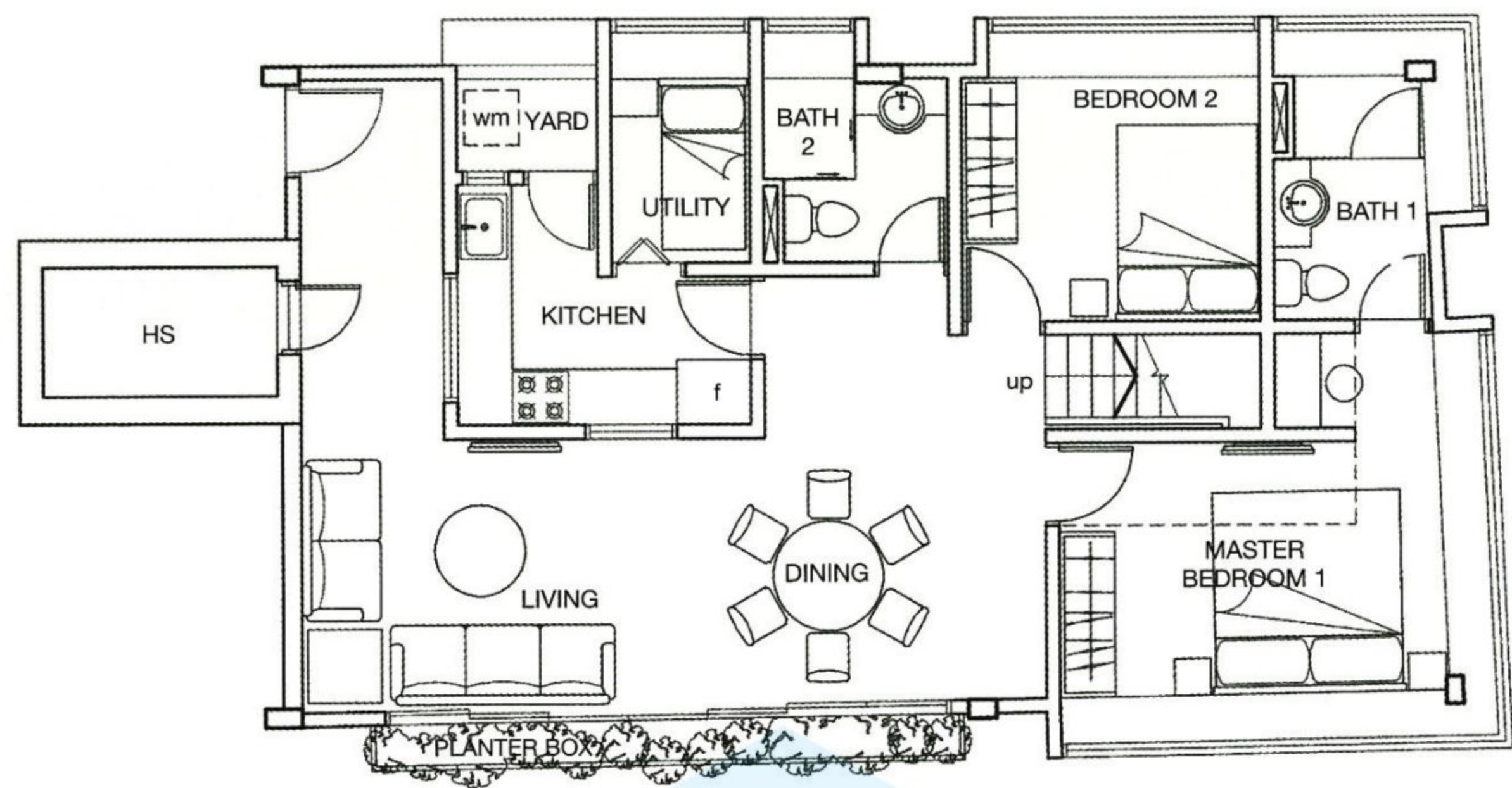
Lower storey
