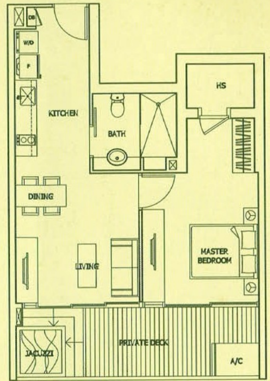
TYPE A2P #01-01 Unit Area 62 sq.m. (667 sq.ft.)
