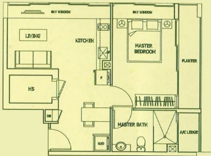
TYPE A3 #02-04 - #04-04
