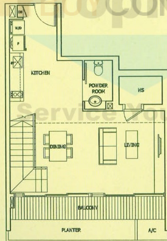
TYPE A2PH (lower) #05-01 Unit Area 116 sq.m. (1249 sq.ft.)
