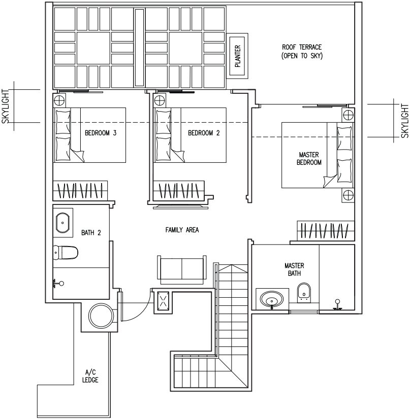
Attic
