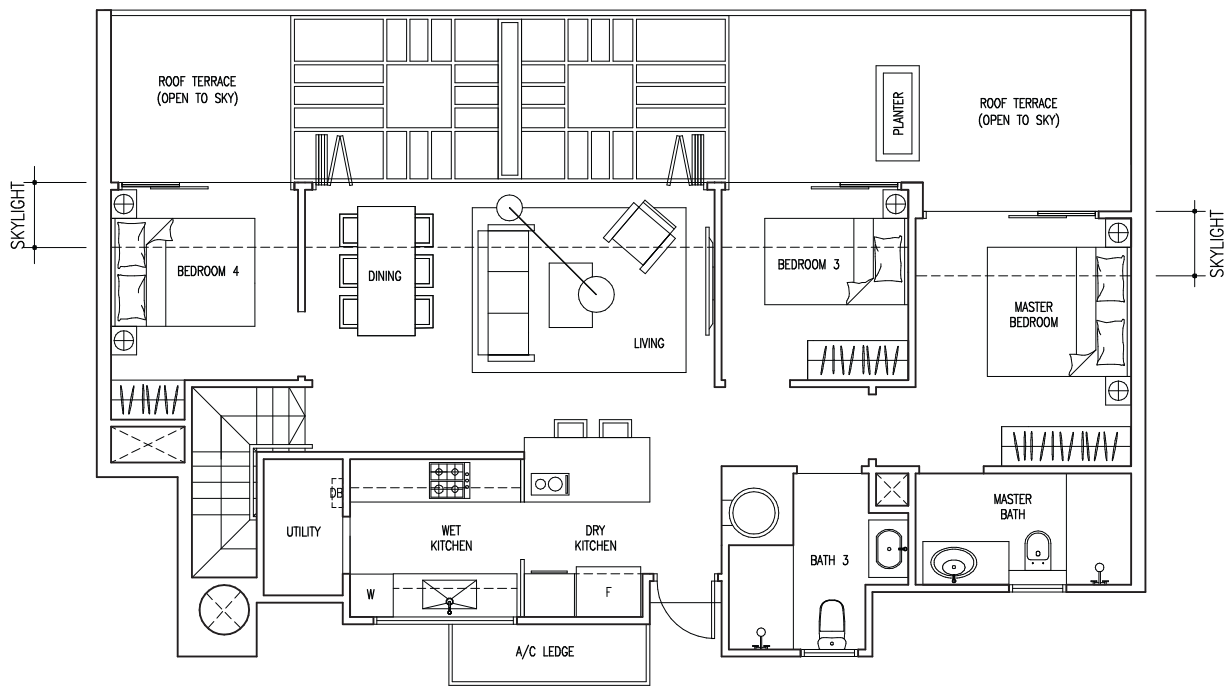
Attic
