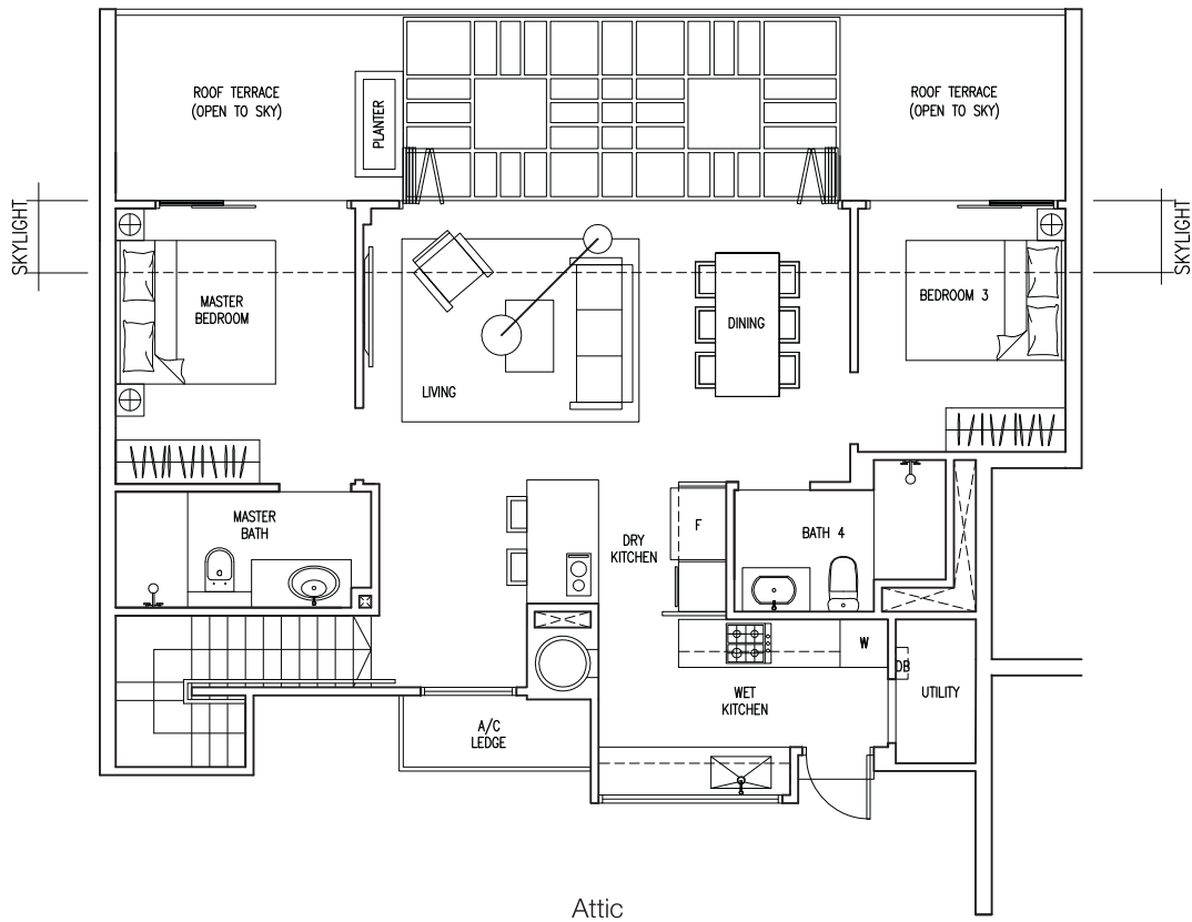
Attic
