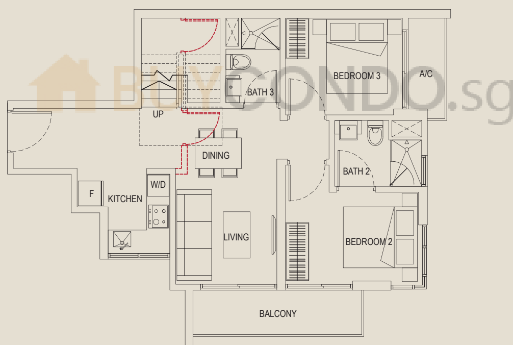
LOWER FLOOR
