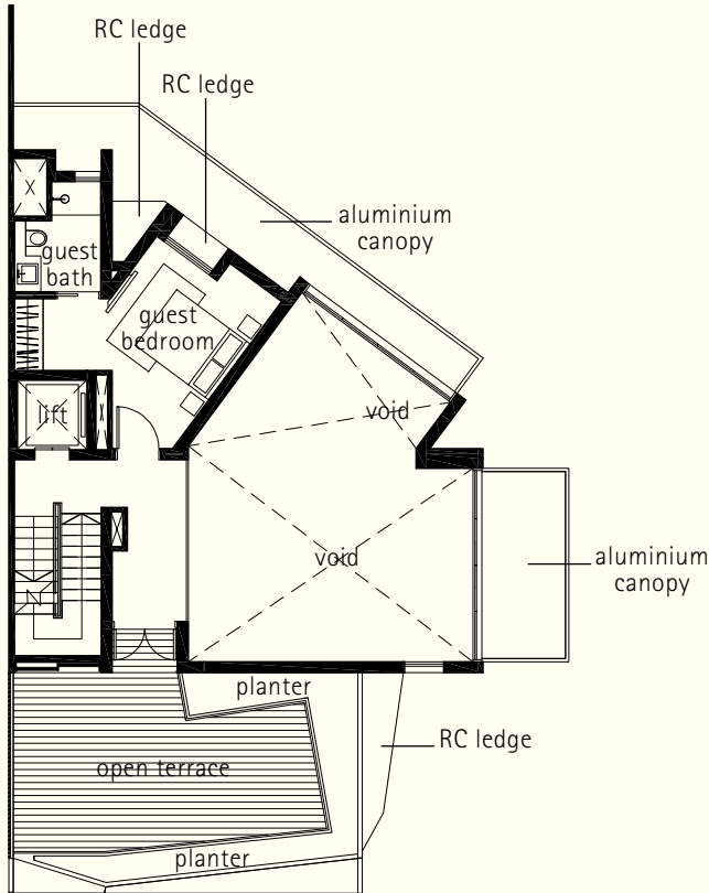
1st storey mezzanine
