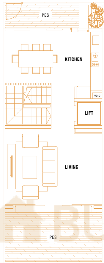
1ST STOREY
