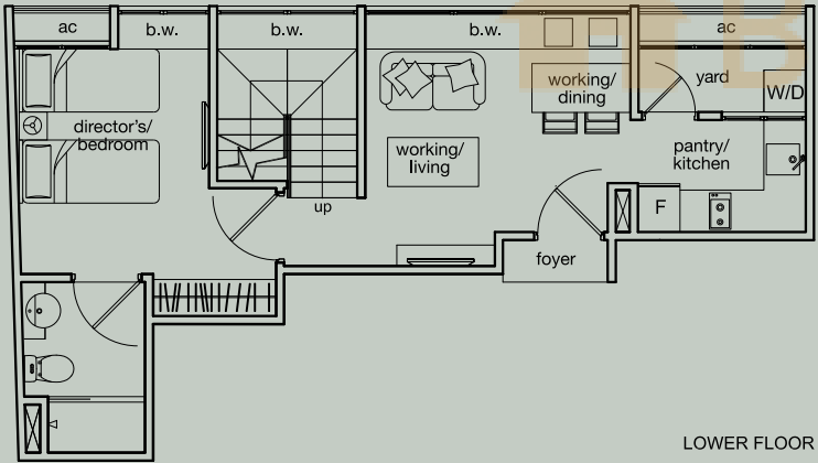
LOWER FLOOR
