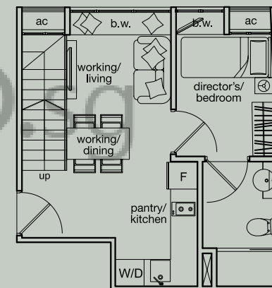
LOWER FLOOR
