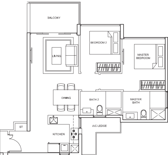
TYPE B2 Area : 71 sq.m Unit(s) : #02-30 to #15-30 #02-38 to #15-38
