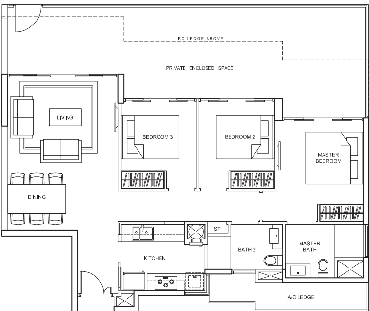
TYPE C1P1 Area : 123 sq.m Unit(s) : #01-01 #01-05 #01-08 (mirror image) #01-09
