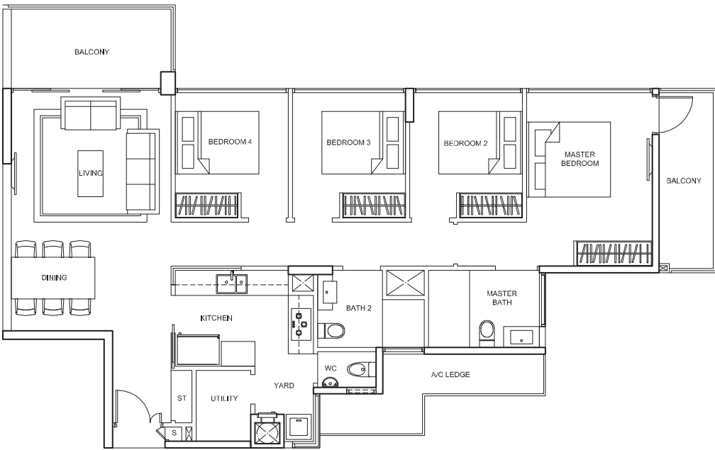
TYPE D3 Area : 125 sq.m Unit(s) : #02-16 to #15-16
