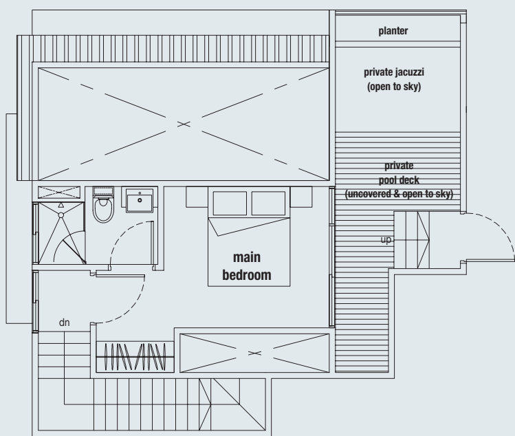
Upper level
