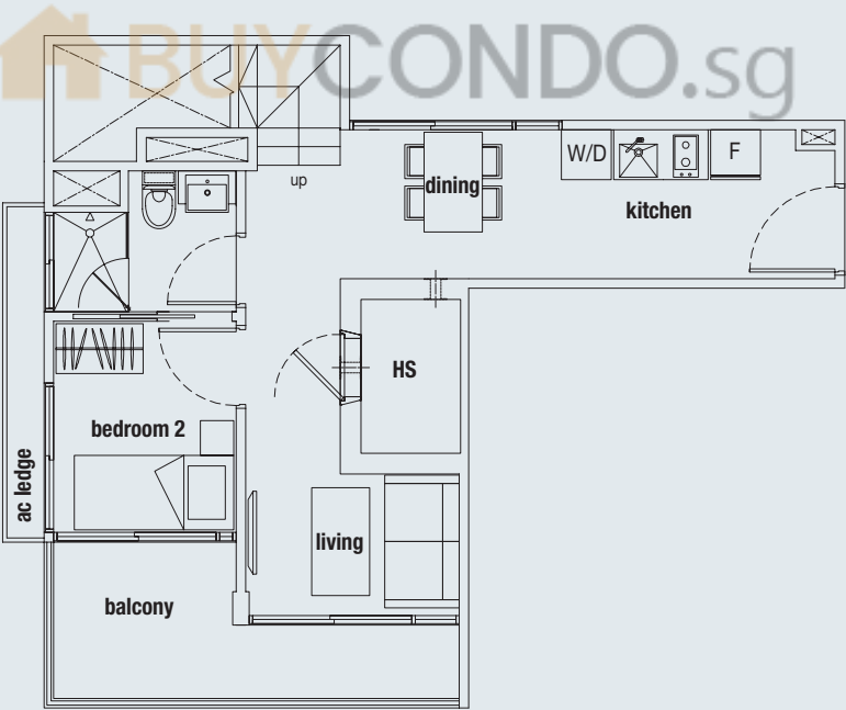
Lower level
