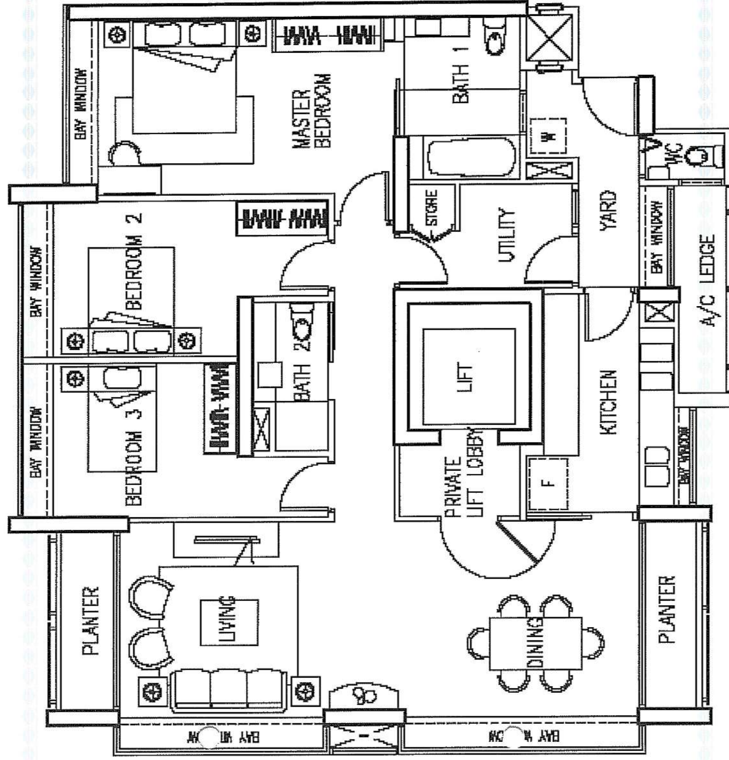
Type C4 APPROX. AREA 136 SQ M | 1464 SQ FT
