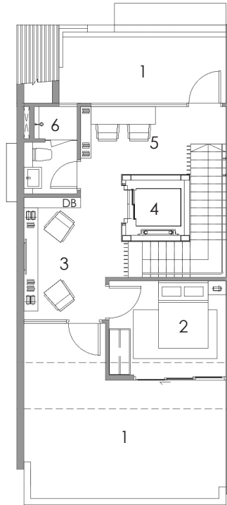
ATTIC PLAN
