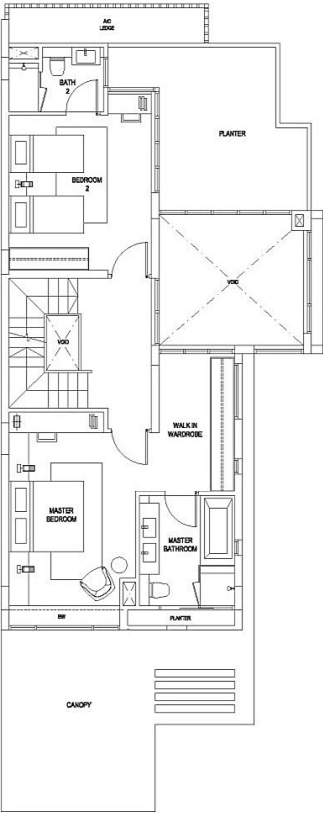
2ND STOREY PLAN
