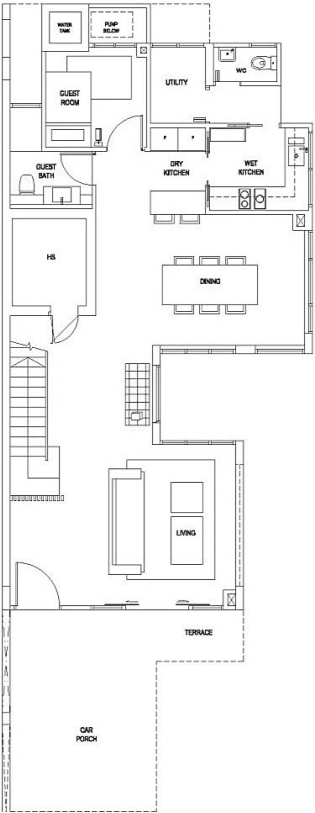
1ST STOREY PLAN
