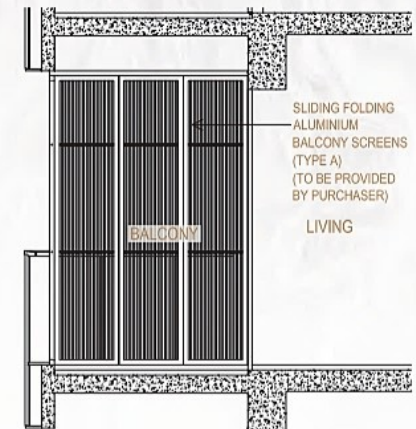
TYPICAL RETRACTABLE BALCONY SCREENING SECTION
