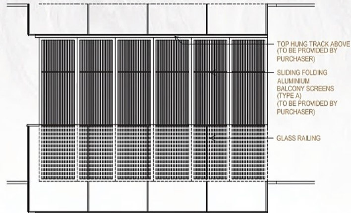
TYPICAL RETRACTABLE BALCONY SCREENING FRONT ELEVATION
