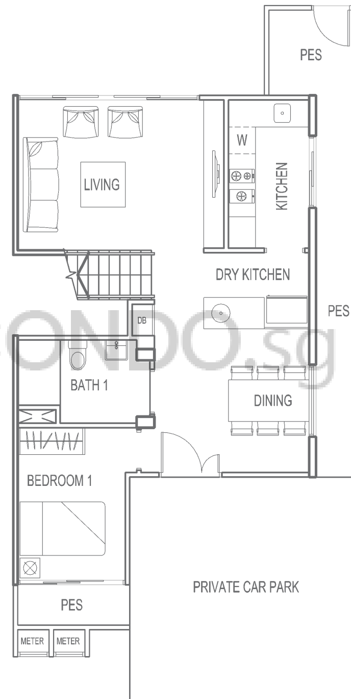
1ST STOREY
