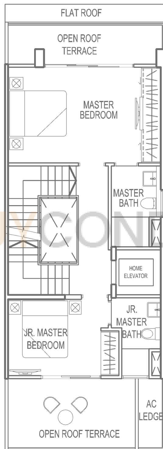
3RD STOREY
