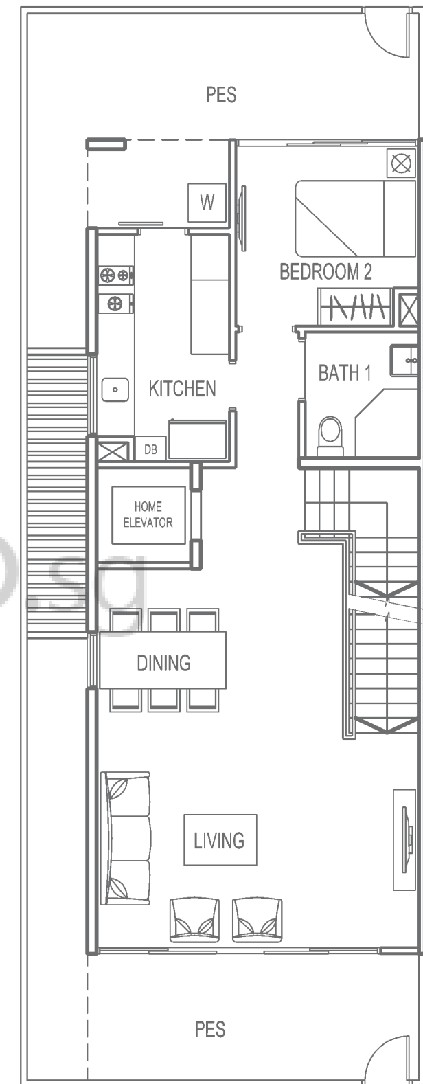
1ST STOREY
