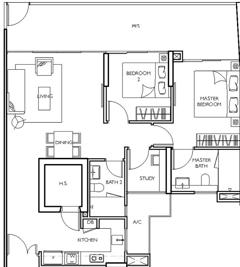
TYPE B2p1 104 sq.m. / 1119 sq.ft.
