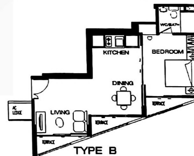
TYPE B #02-01 46 sqm / 495 sqft
