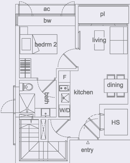
LOWER FLOOR
