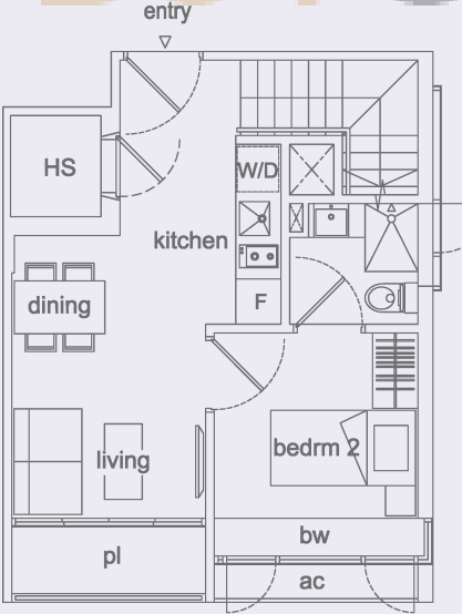
UPPER FLOOR
