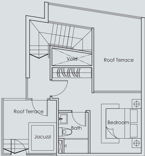
UPPER LEVEL
