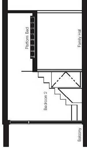
SECTION X-X
