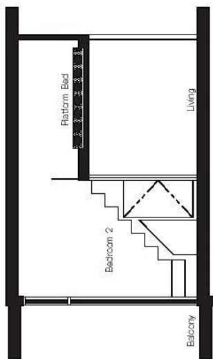
SECTION X-X
