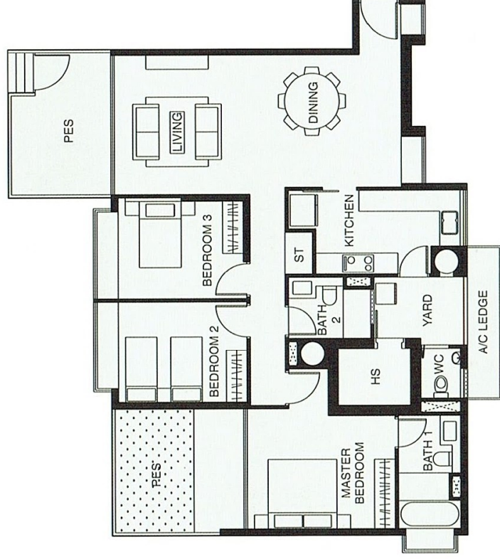
TYPE B8 155 sq m (1,668 sq ft) #01-05
