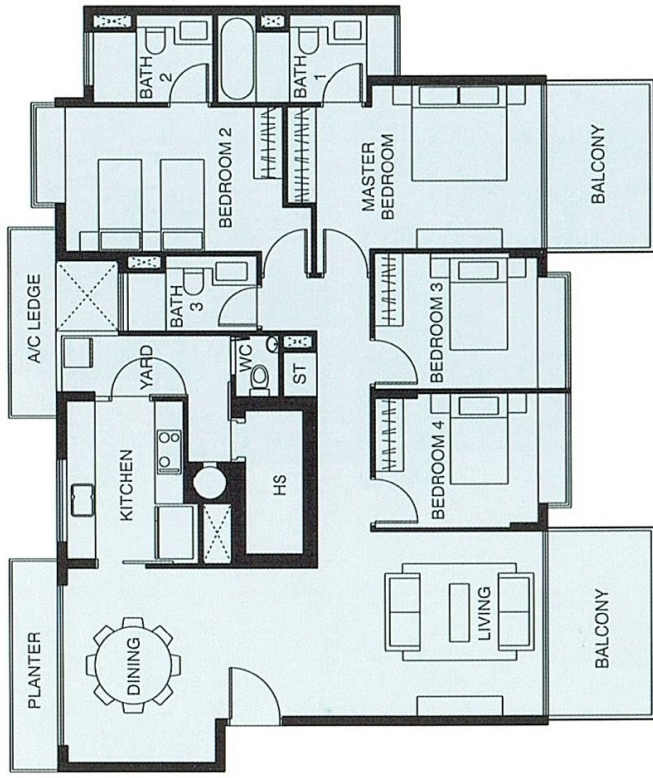
TYPE C3 171 sq m (1,841 sq ft) #16-07 – #17-07
