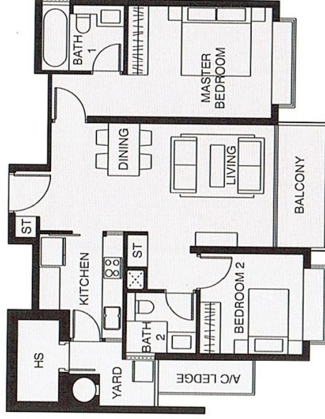
TYPE A3 91 sq m (980 sq ft) #05-06 – #12-06
