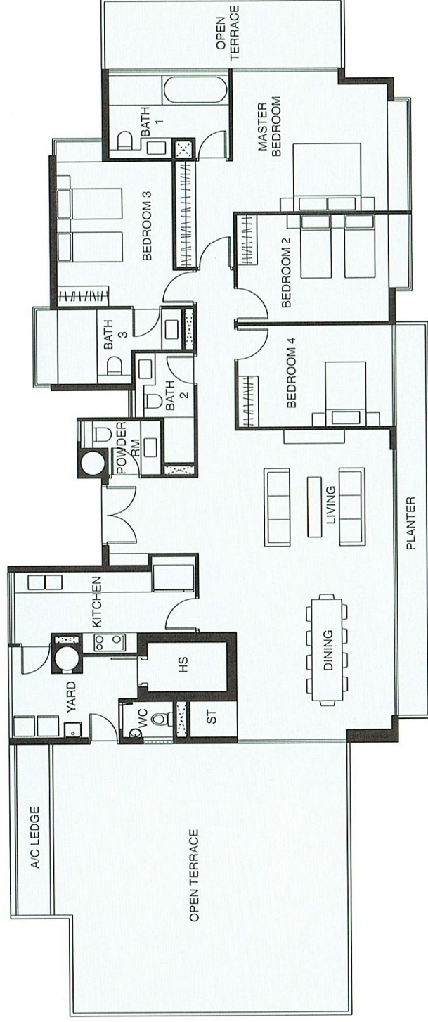
TYPE P1 298 sq m (3,208 sq ft) #18-03
