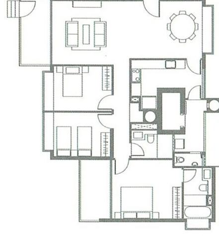
TYPE B9(m) 146 sq m (1,572 sq ft) #01-08
