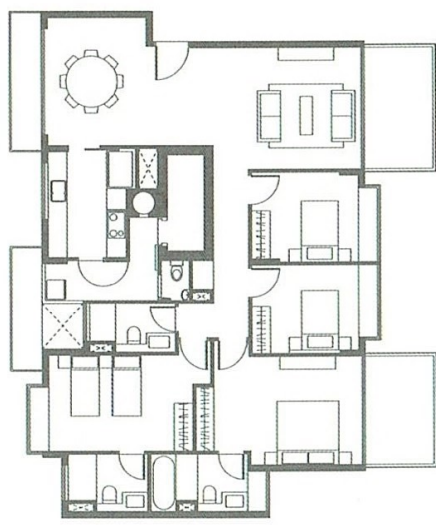
TYPE C3(m) 171 sq m (1,841 sq ft) #16-08 – #17-08
