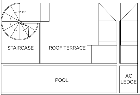
ROOF TERRACE
