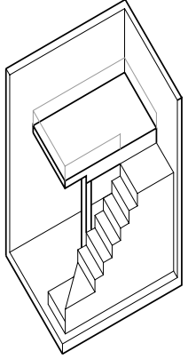
ISOMETRIC VIEW Floor Height: 3600mm
