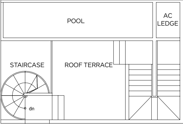
ROOF TERRACE
