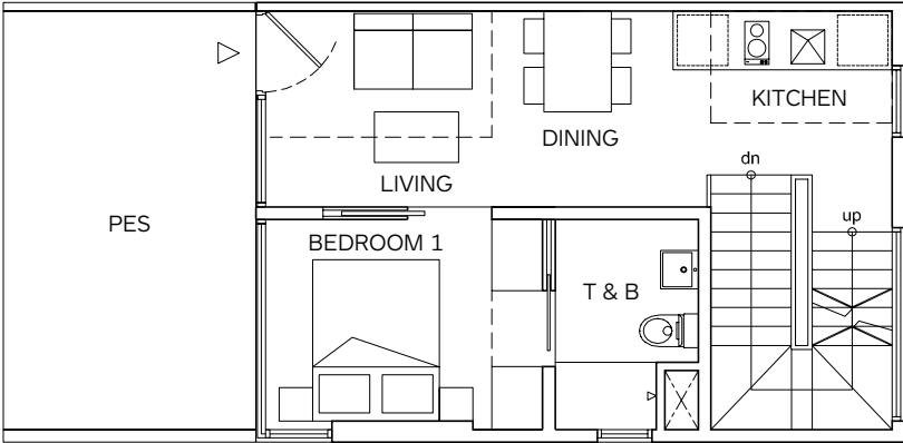
2ND STOREY
