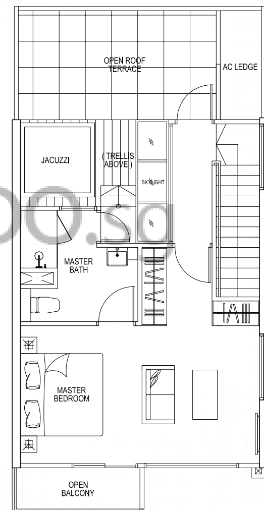
5TH STOREY PLAN
