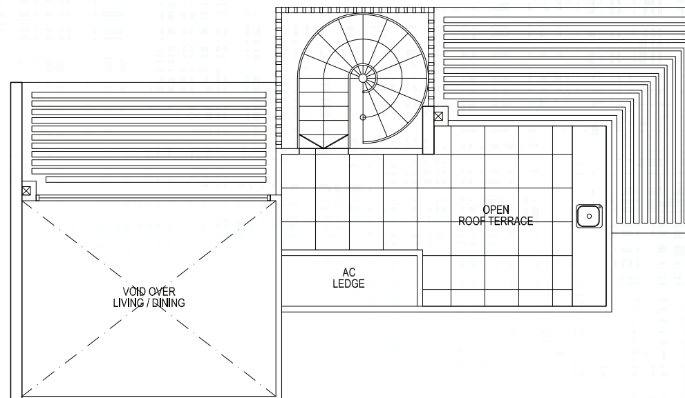
ROOF PLAN
