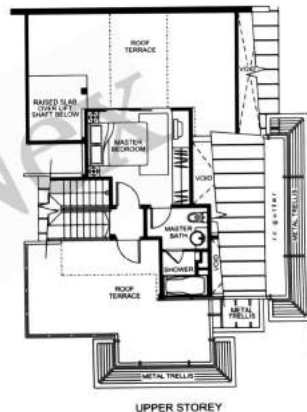
UPPER STOREY
