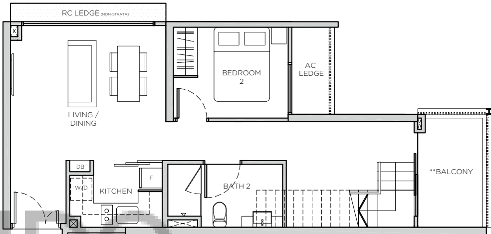
LOWER LEVEL
