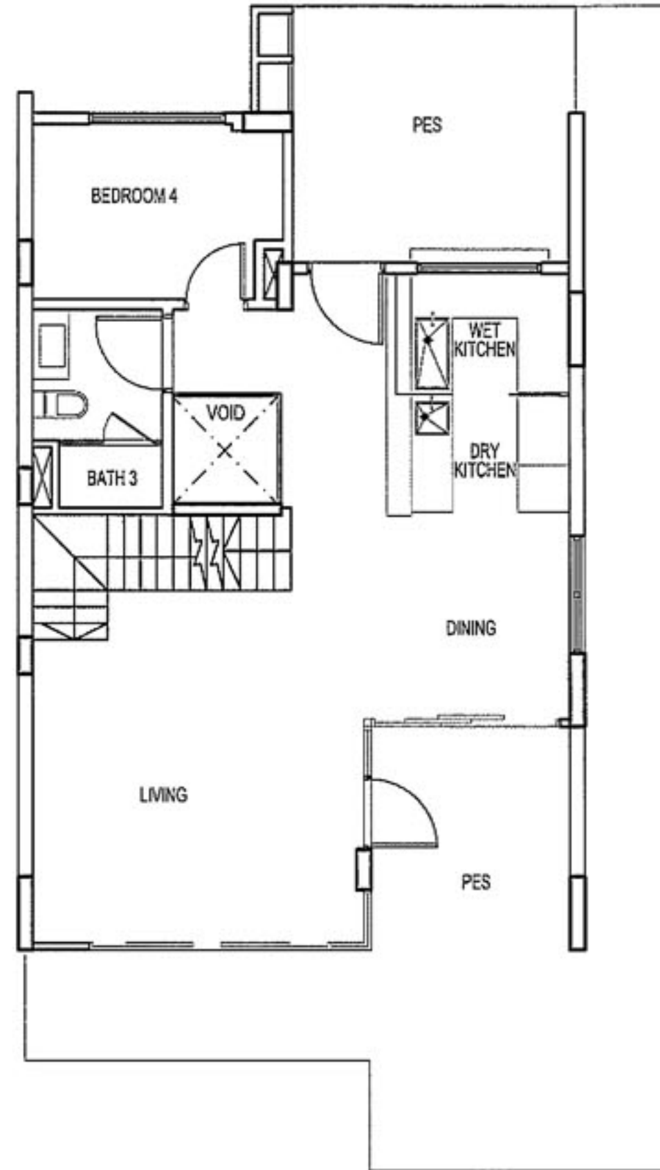
1ST STOREY PLAN
