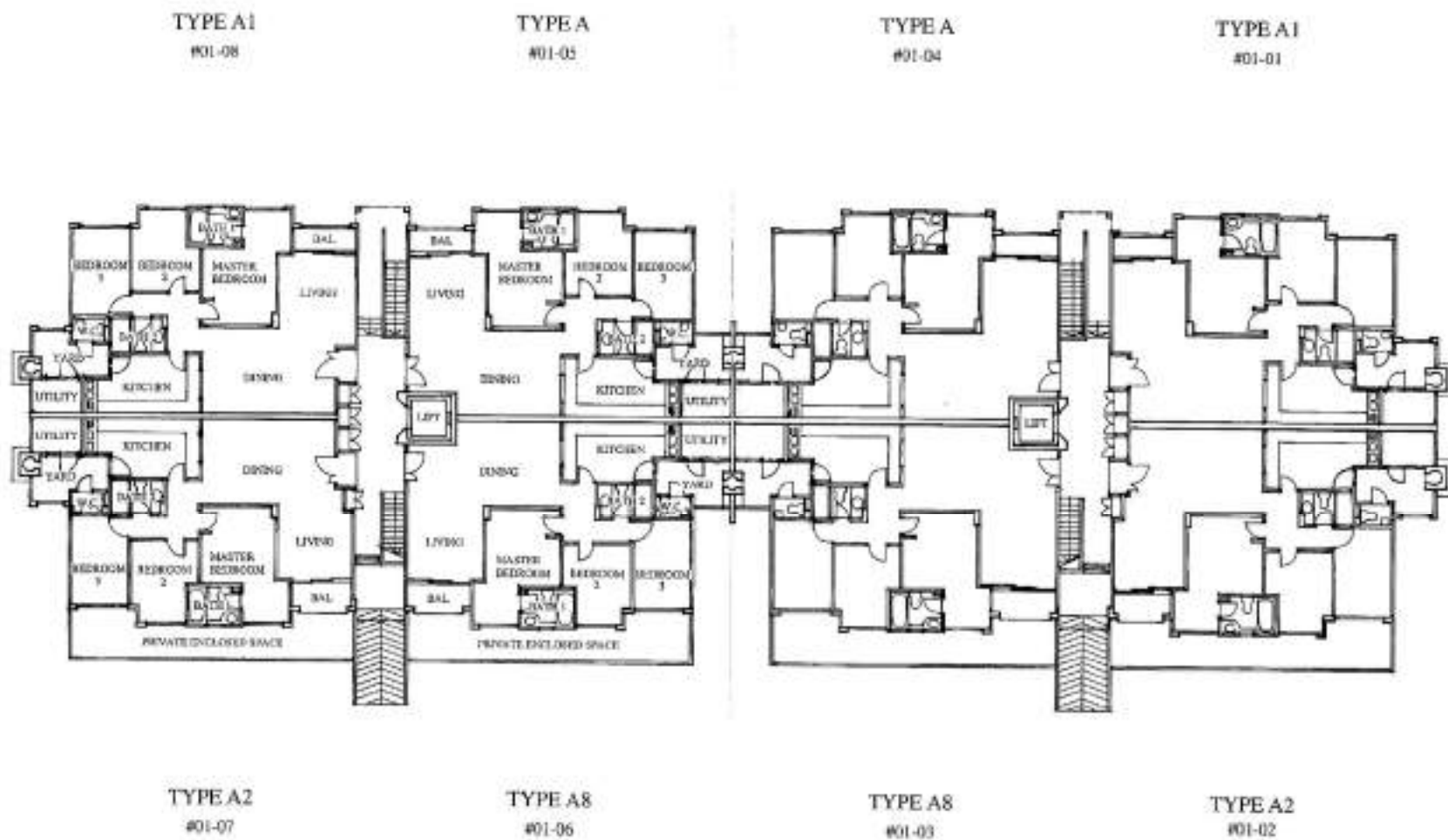
1ST STOREY PLAN – TOWERS 2 & 3
