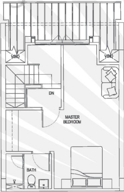
ATTIC
