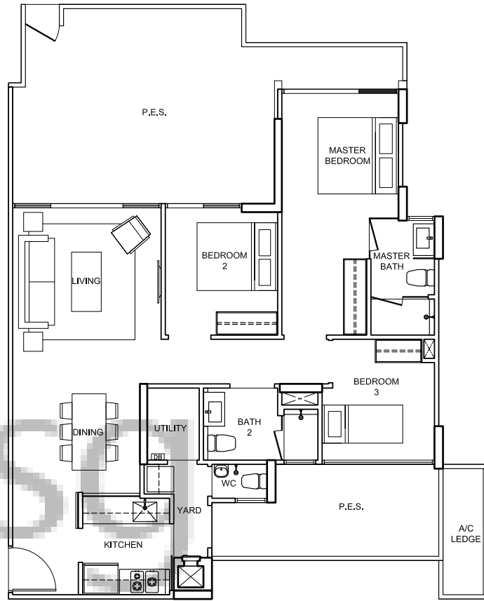
TYPE C3b-pes-02 130 sqm/ 1,402 sq ft 80, Elias Road # 01 - 02
