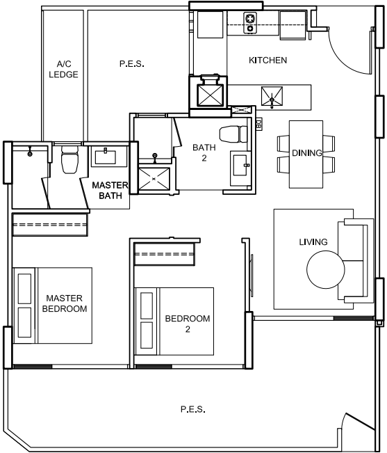
TYPE B3-pes-02 89 sqm/ 960 sq ft 90, Elias Road # 01 - 33
