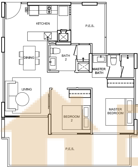
TYPE B2-pes-02 88 sqm/ 949 sq ft 82, Elias Road # 01 - 09
