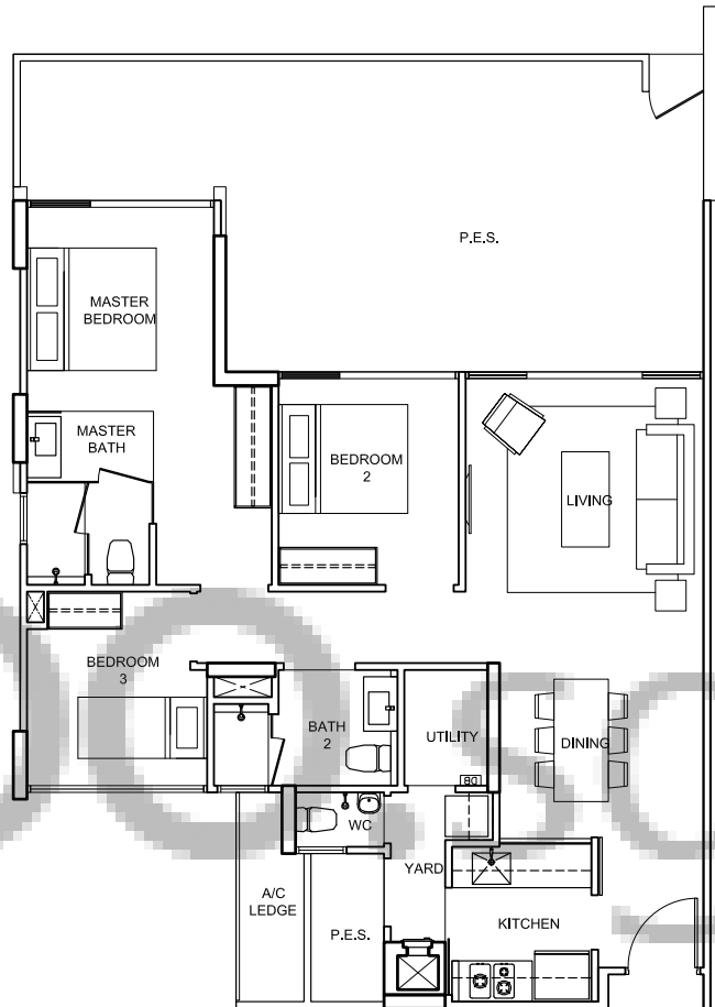
TYPE C1a-pes-01 130 sqm/ 1,402 sq ft 86, Elias Road # 01 - 18 # 01 - 19 100, Elias Road # 01 - 62
