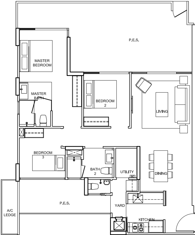
TYPE C1b-pes-02 130 sqm/ 1,402 sq ft 92, Elias Road # 01 - 39
