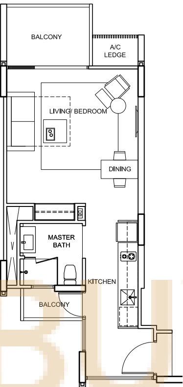
TYPE A2 46 sqm/ 497 sq ft 98, Elias Road # 05 - 53 # 04 - 53 # 03 - 53 # 02 - 53
