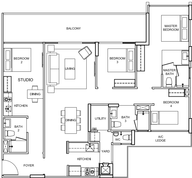
TYPE D4 137 sqm/ 1,477 sq ft 88, Elias Road # 04 - 24 # 04 - 25 # 03 - 24 # 03 - 25 # 02 - 24 # 02 - 25
