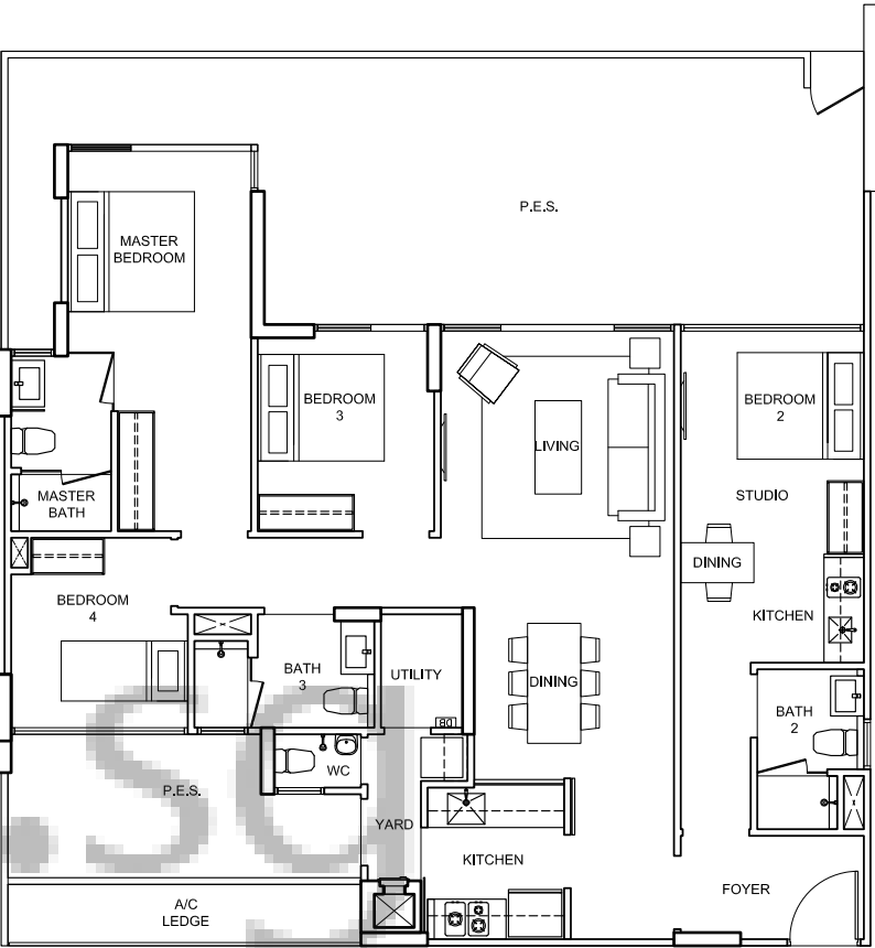
TYPE D7-pes 172 sqm/ 1,853 sq ft 88, Elias Road # 01 - 28
