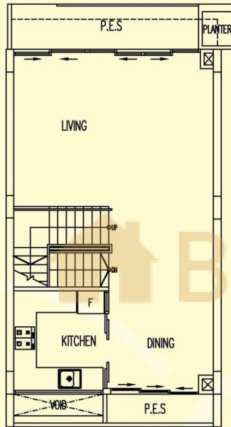
1ST STOREY
