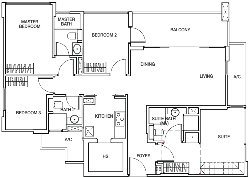
4 bedroom layout
