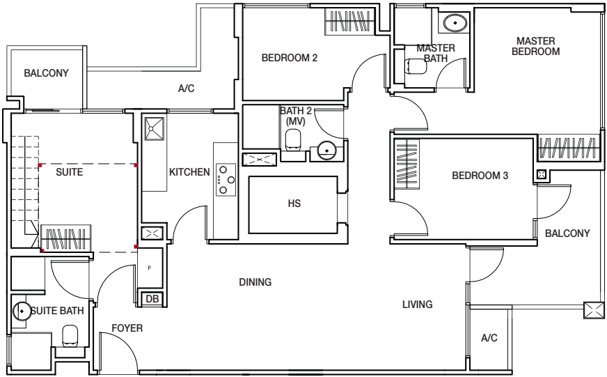
4 bedroom layout
