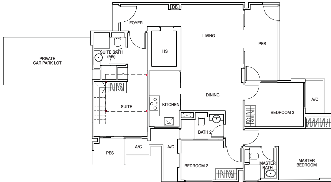
4 bedroom layout
