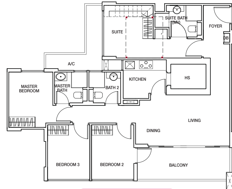
4 bedroom layout
