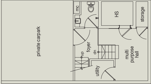
basement
