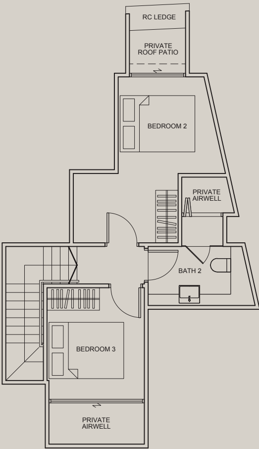
Upper level
