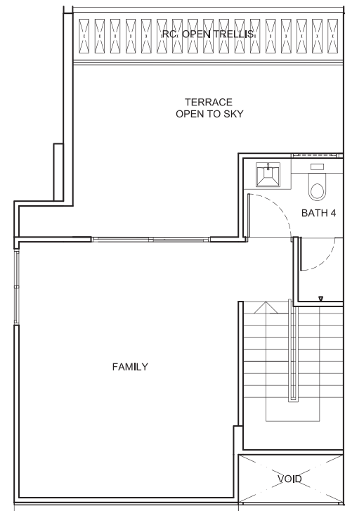
ATTIC
