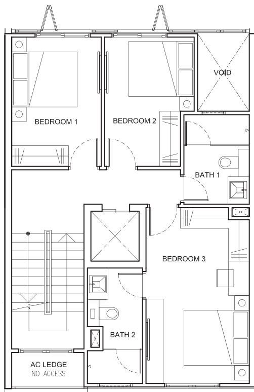
SECOND STOREY
