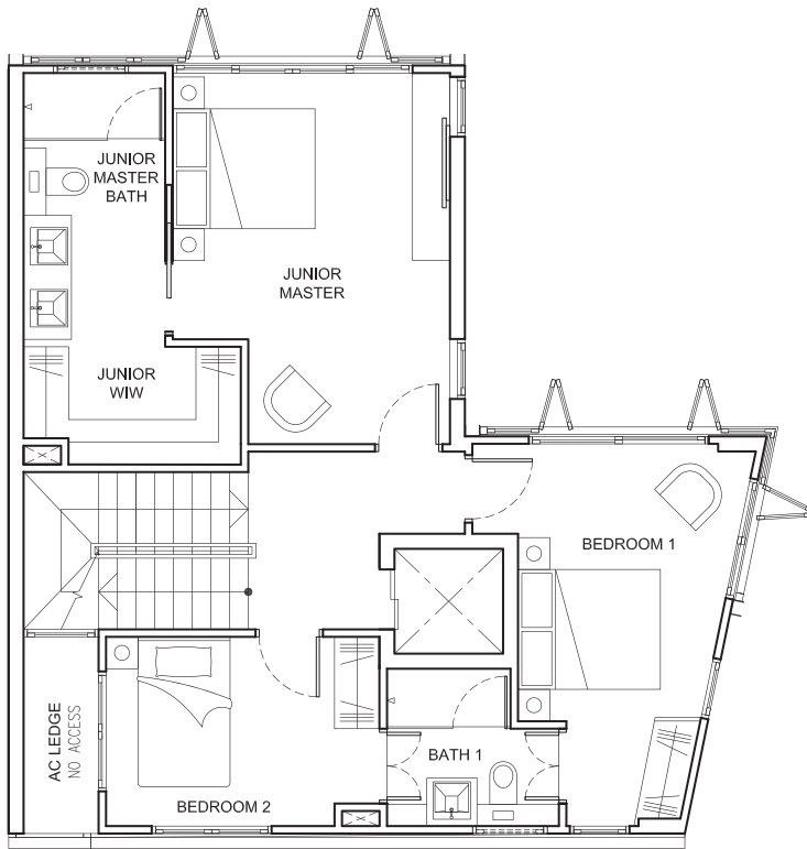
SECOND STOREY
