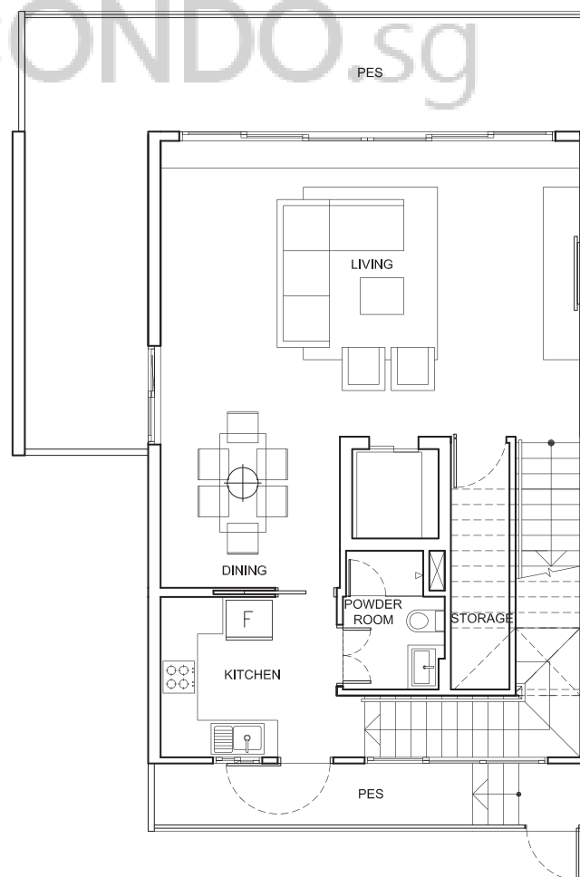
FIRST STOREY
