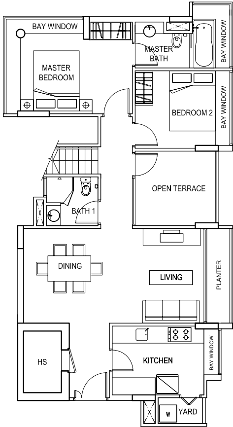
LOWER STOREY
