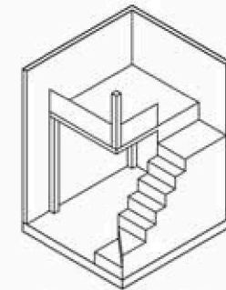
ISOMETRIC OF FURNITURE PLATFORM
