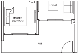
TYPE Bs2-P 60 sq m/ 646 sq ft #01-32
