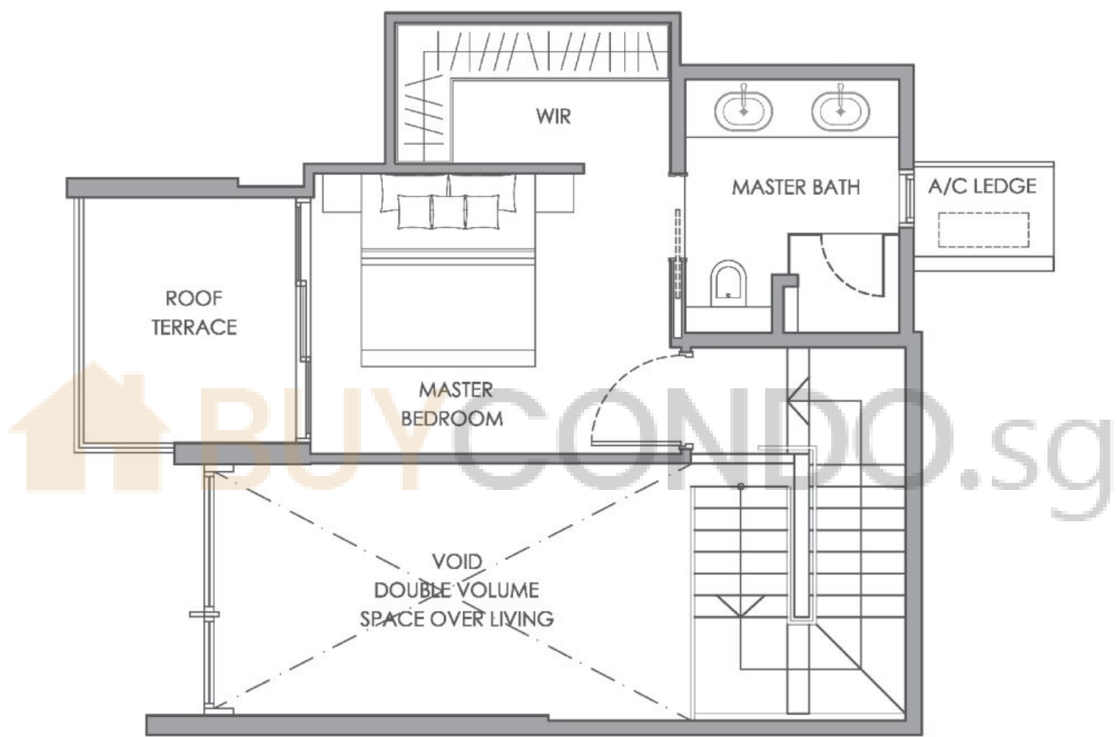
UPPER PLAN
