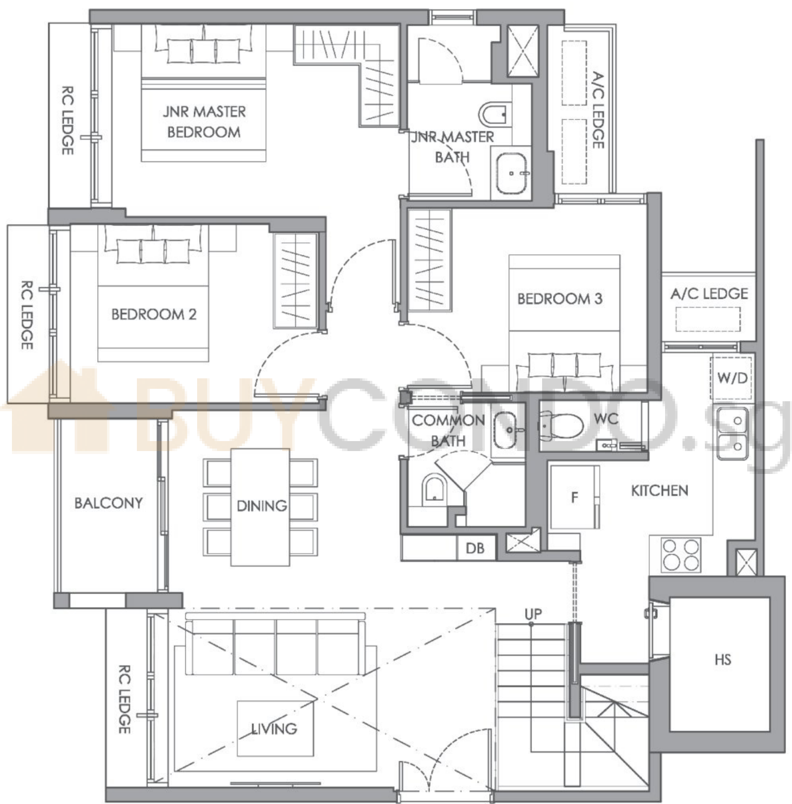
LOWER PLAN
