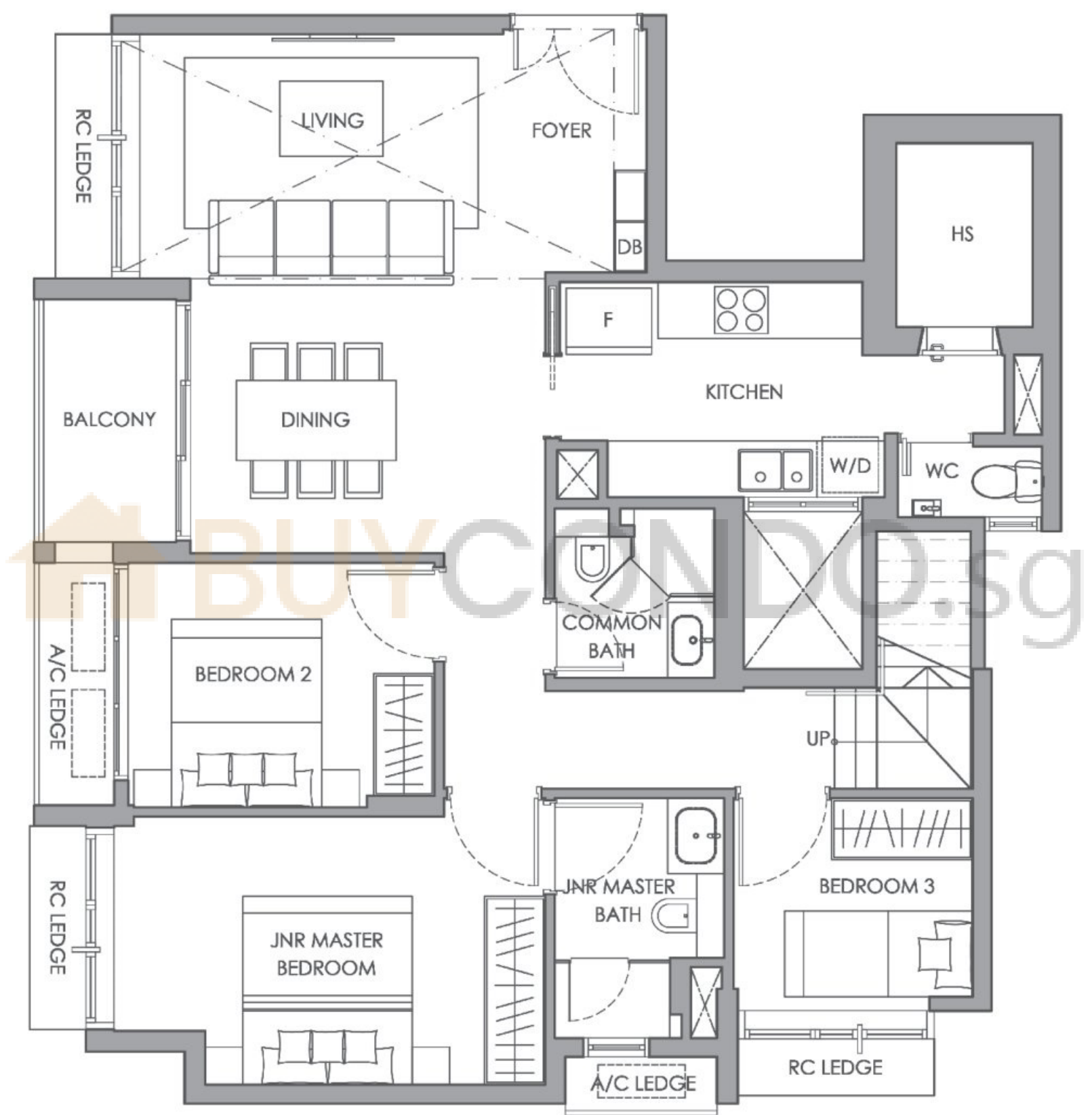
LOWER PLAN
