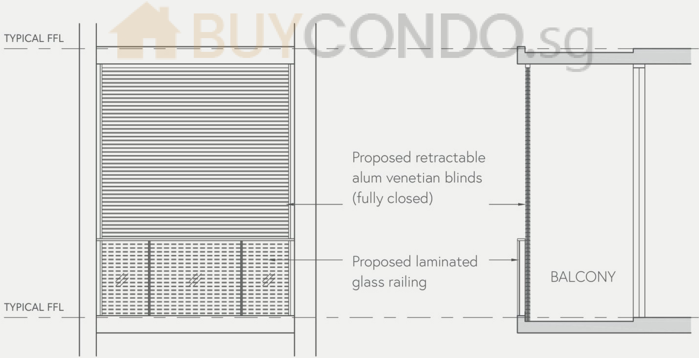
FRONT ELEVATION
