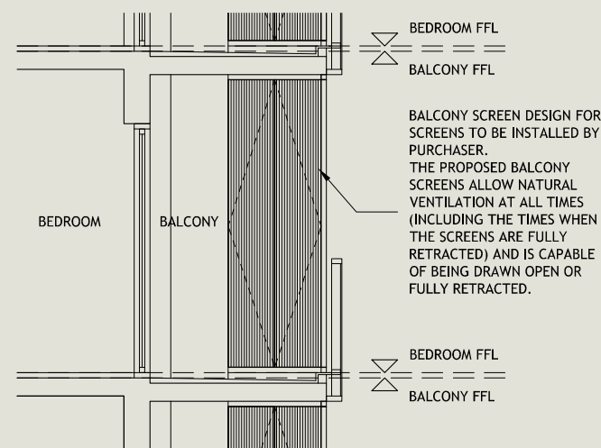
TYPICAL SECTION
