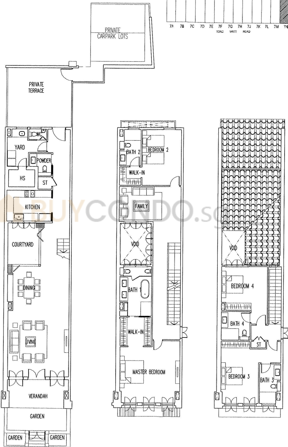
1st Storey
