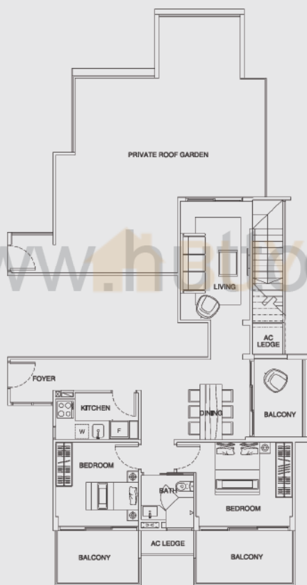
5th STOREY
