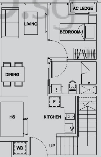
Lower Floor
