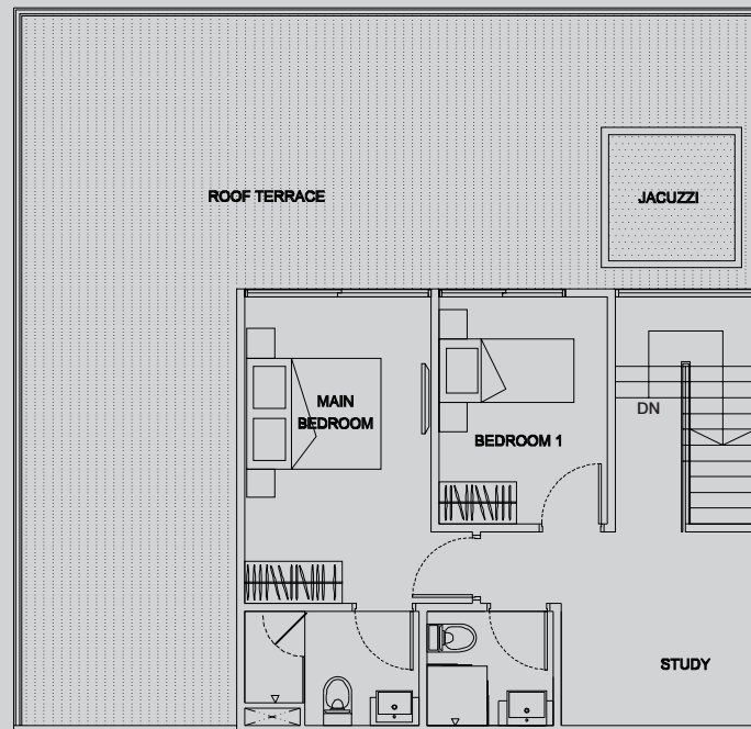
Upper Floor
