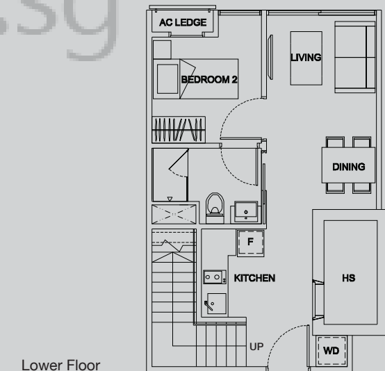
Lower Floor
