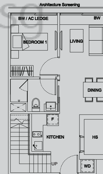
Lower Floor
