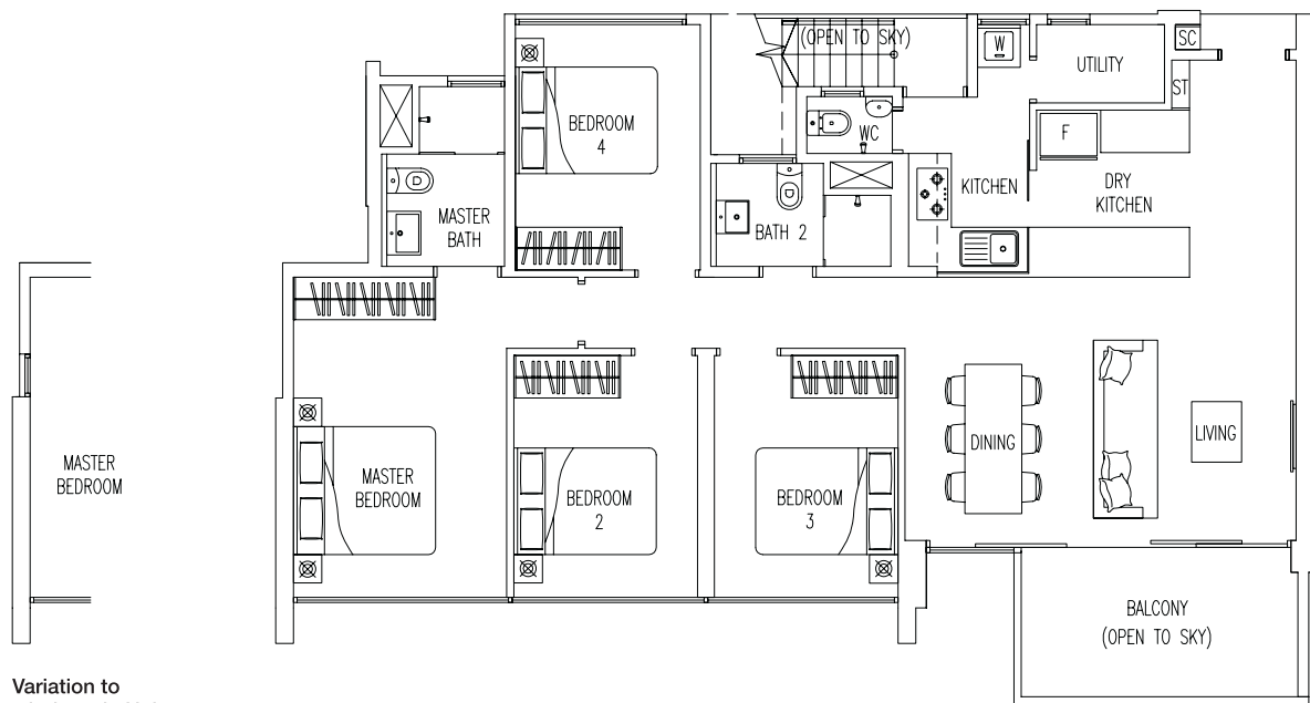
LOWER FLOOR
