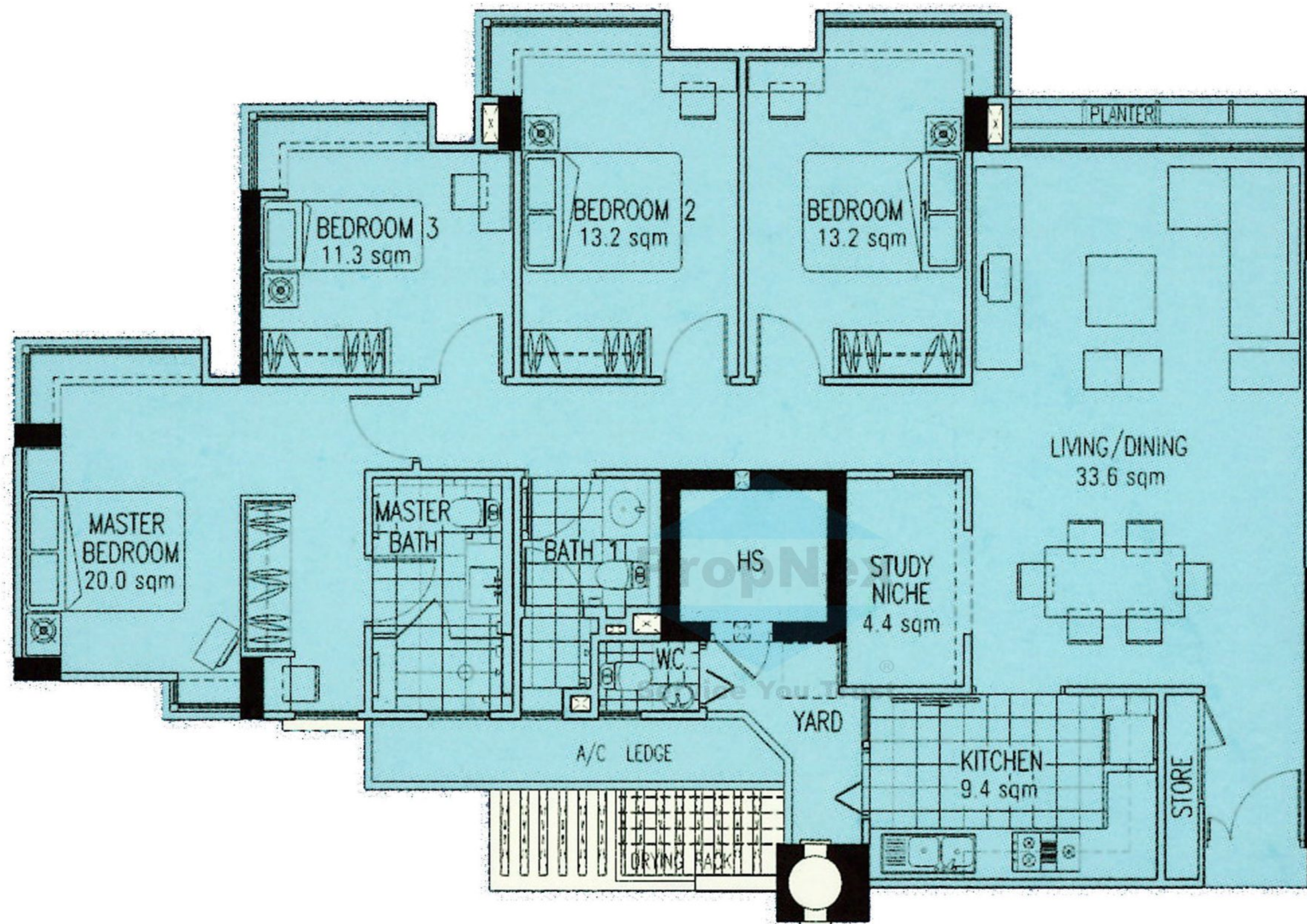
Type E 144 sqm (1550 sqft)
