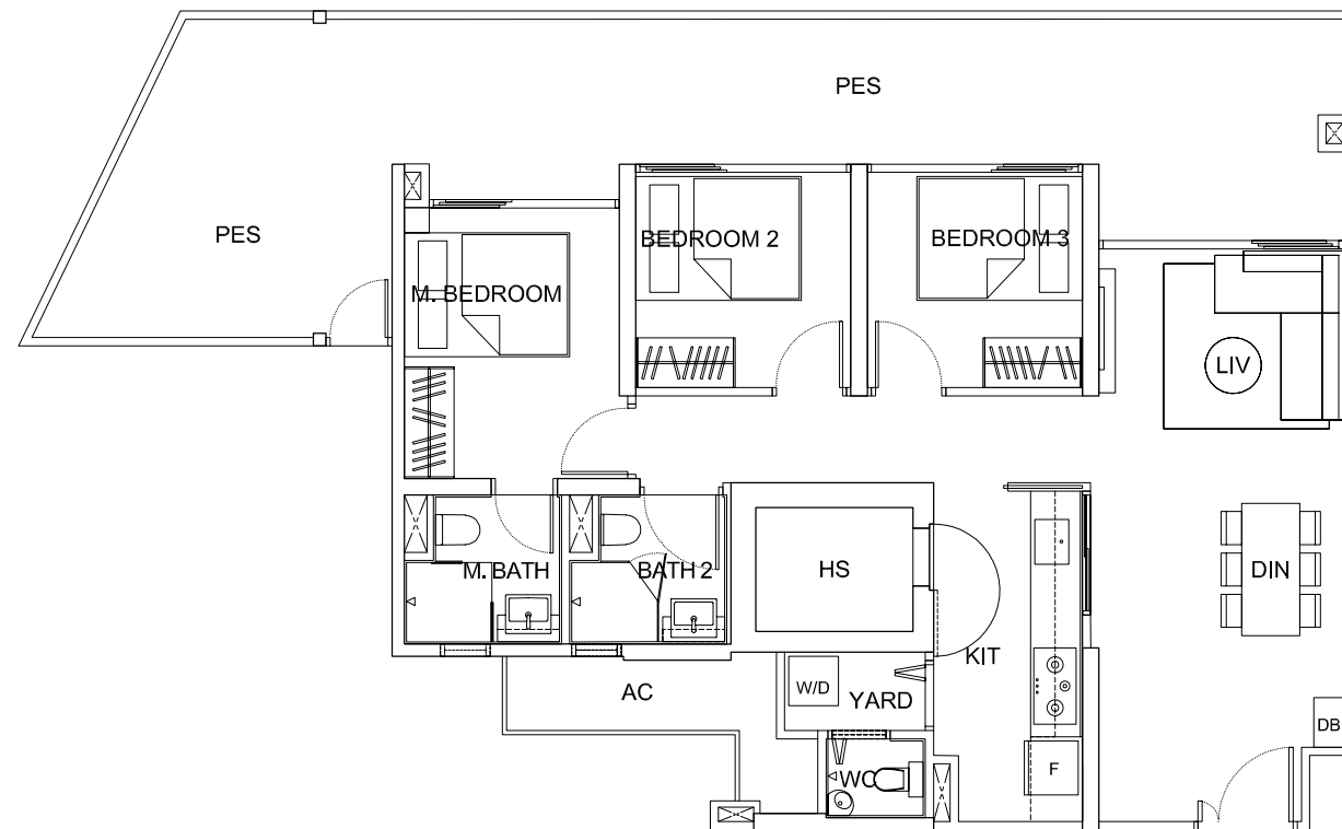
Type C7-P
