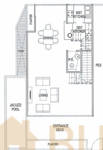
1ST STOREY PLAN
