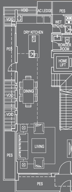
1st Storey Plan
