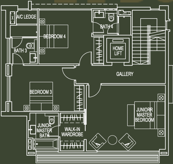
2nd Storey Plan
