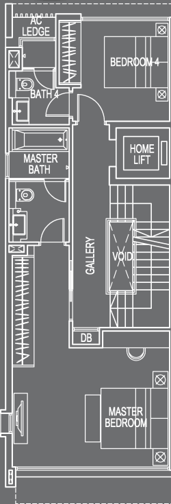
3rd Storey Plan
