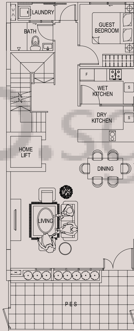
1ST STOREY PLAN
