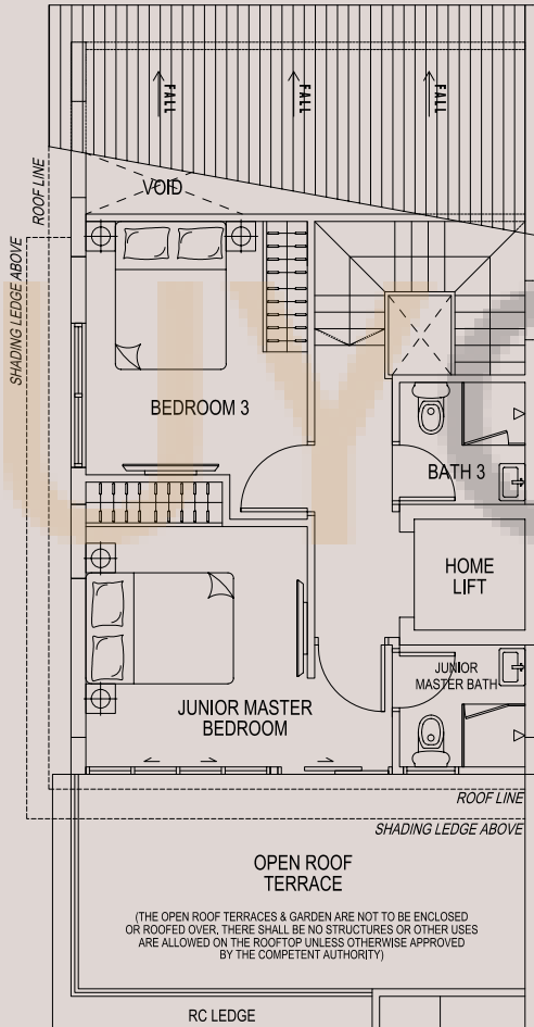
ATTIC PLAN
