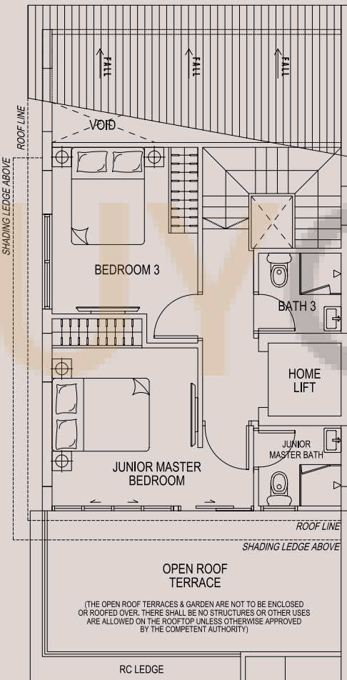
ATTIC PLAN
