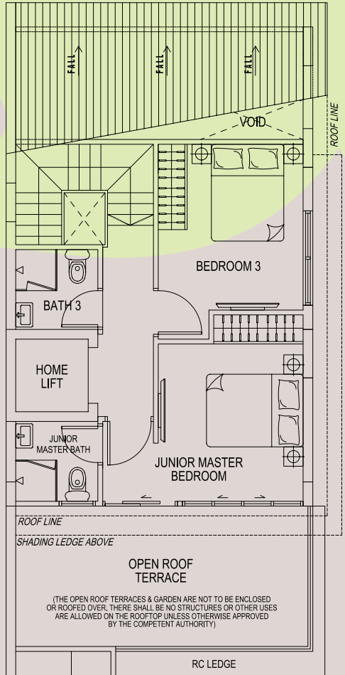
ATTIC PLAN
