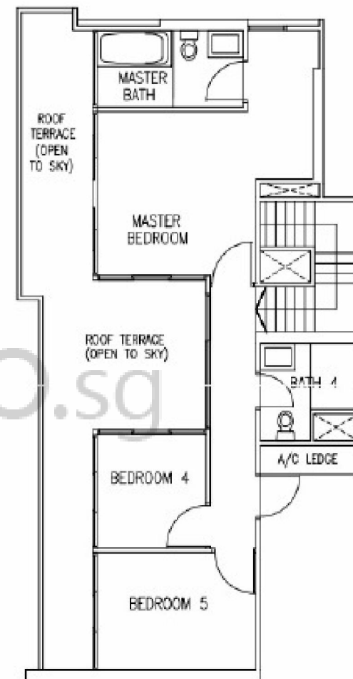
35TH STOREY PLAN
