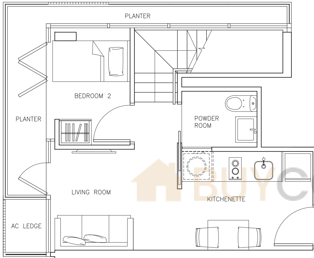
LOWER PENTHOUSE #10-05
